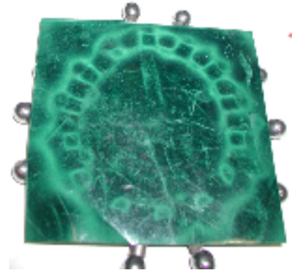
Dumbbell Atom as seen on magnetic viewing paper
