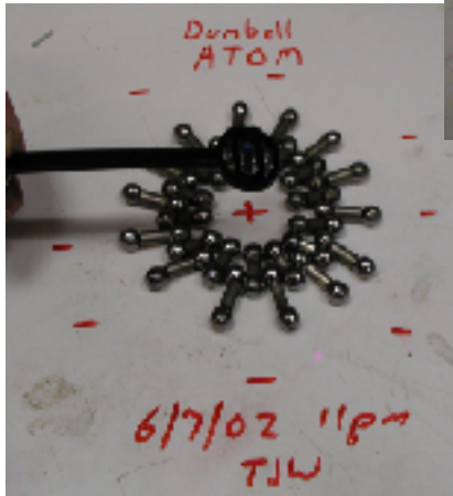
Uniform (Sp,+) "Nucleus" Center
