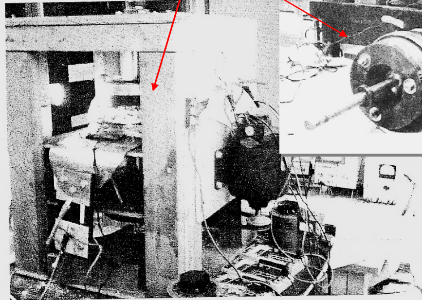
Figure 12. Homopolar generator - rotating. Square wave on Oscilloscope is the photocell circuit output.
