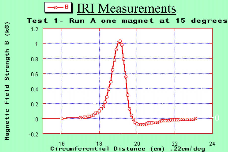
Asymmetric gaussmeter data plot
